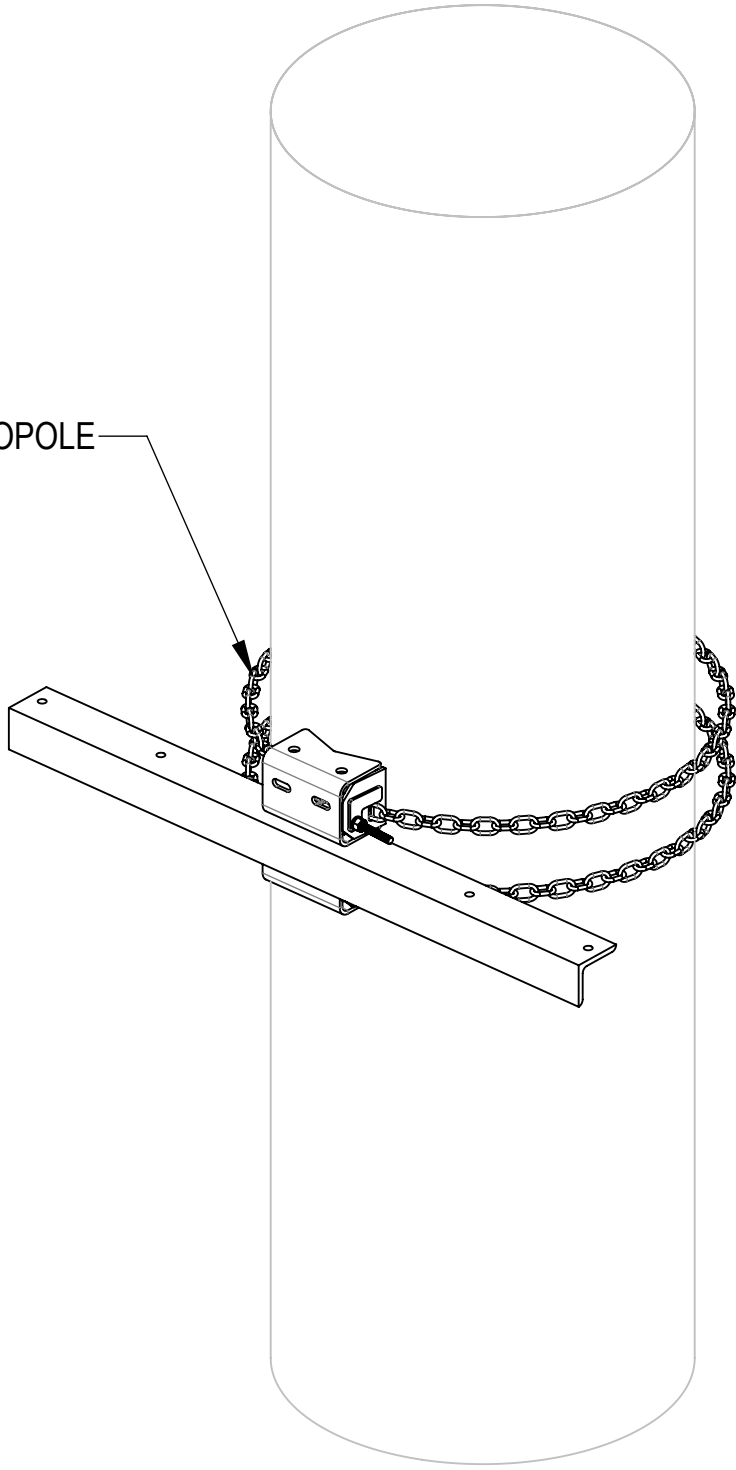
ATTACHED TO MONOPOLE VIEW
