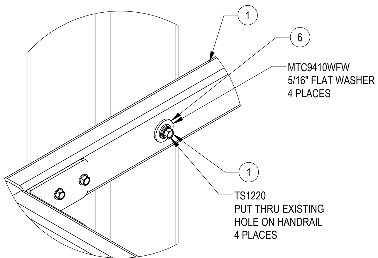
DETAIL J SCALE 1 : 2
