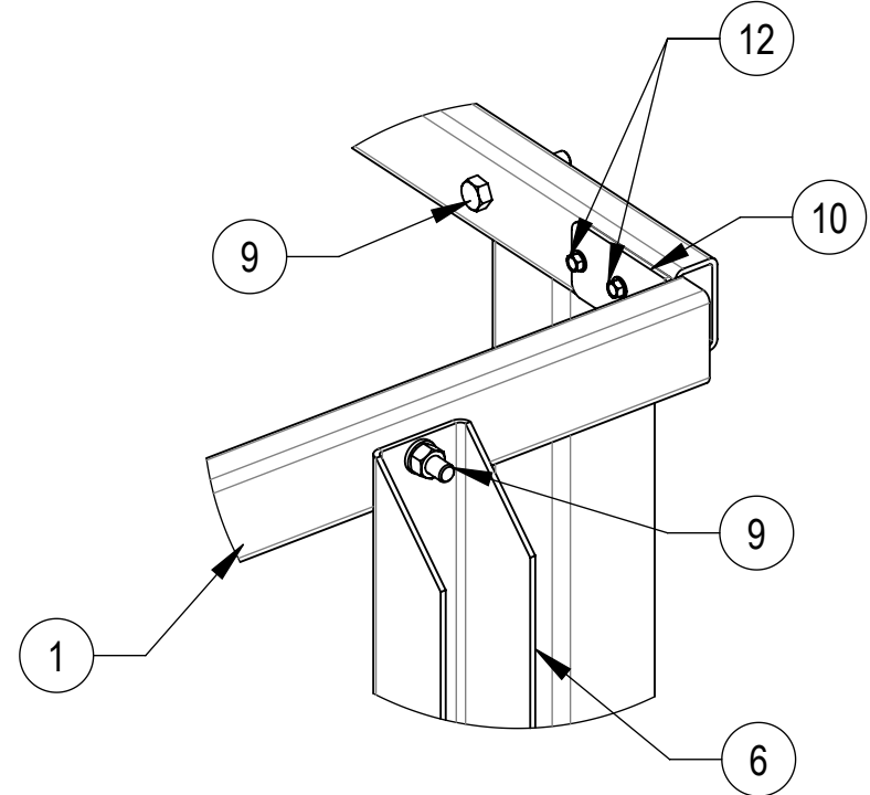
DETAIL E SCALE 1:4
