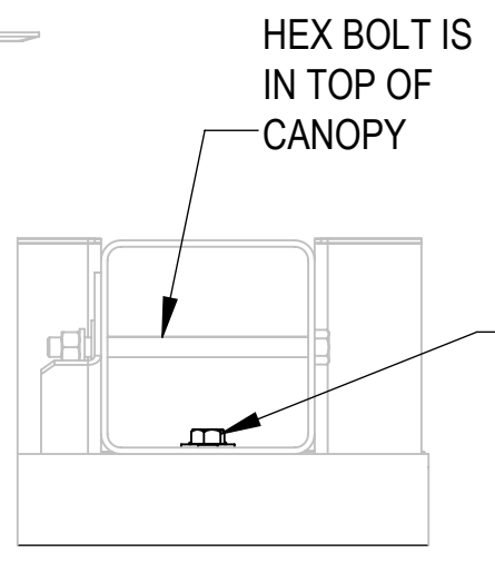
SECTION F-F SCALE 1 : 4
