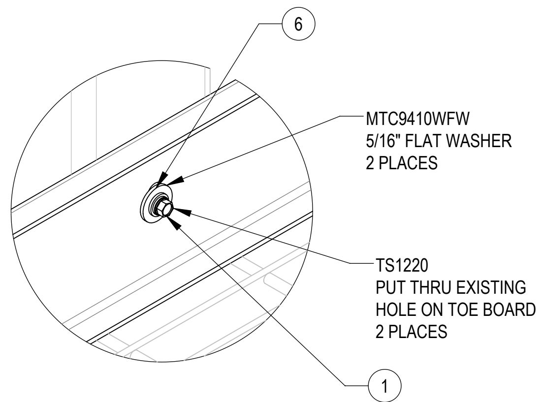
DETAIL K SCALE 1 : 2
